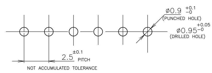
RECOMMENDABLE P.C.BOARD LAYOUT (B.C.B THK:1.0~1.6)
